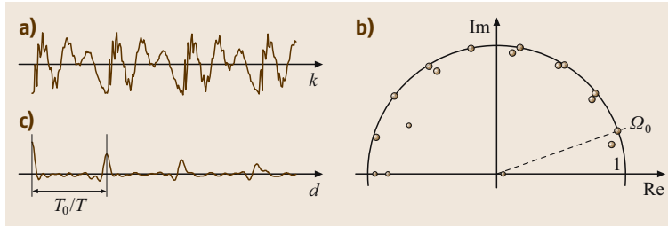
Fig. 10.7a–c PDA with active modeling. (a) Signal: 32 ms, vowel [e], male voice; (b) zeros of the 41-st-order LP polynomial in the z plane (upper half; sampling frequency reduced to 2 kHz); (c) reconstructed impulse response with zero phase and equal amplitude of all partials
